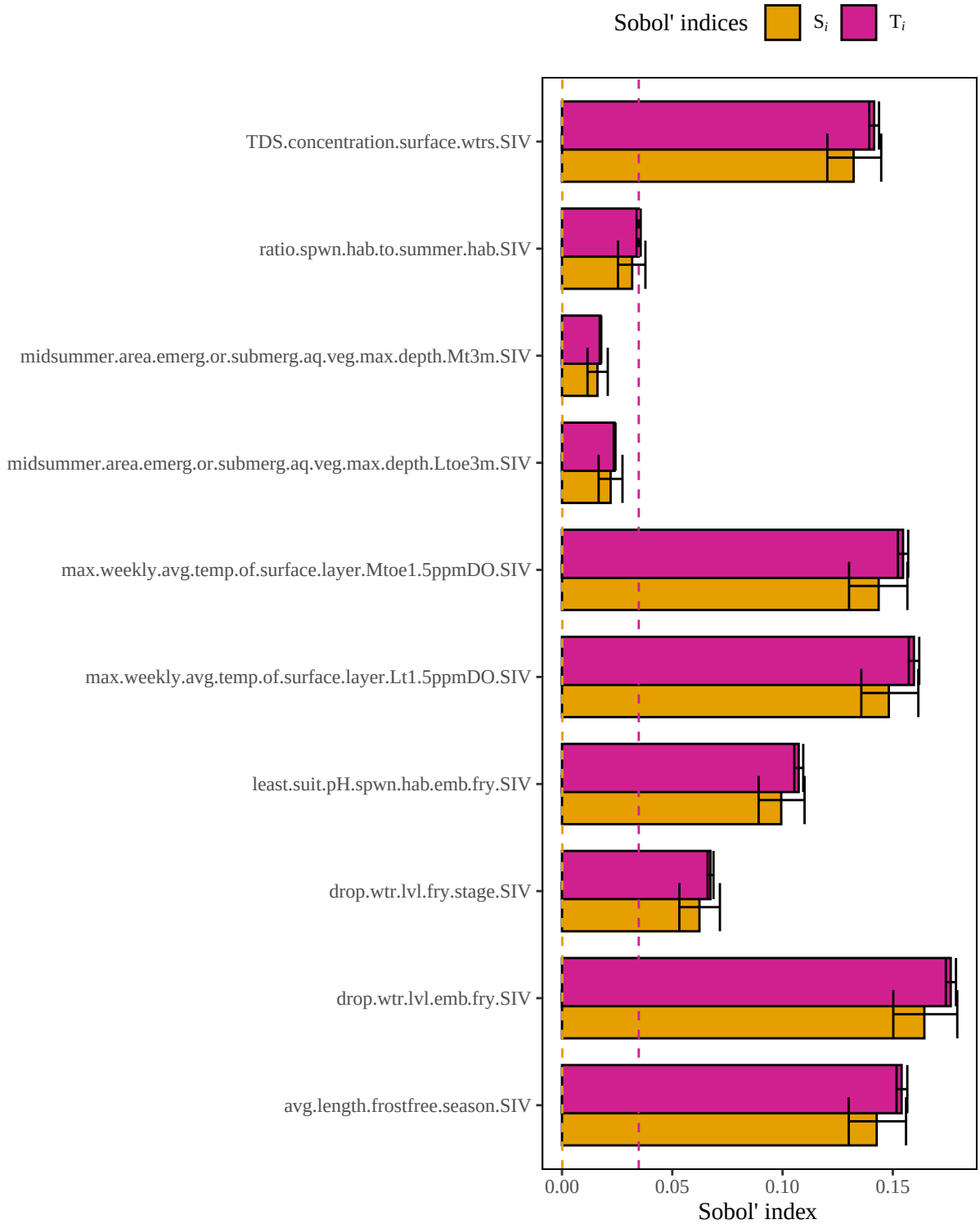
Figure 5. Results of a sensitivity analysis for the northernpikeLacVegD model based on a geometric mean structure. Dashed lines represent baseline numerical approximation error for S_i and T_i ( i.e. , dummy variables).
